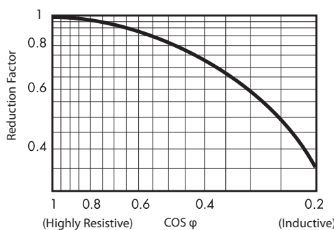
Figure 20 - Load Reduction factor versus cos φ
