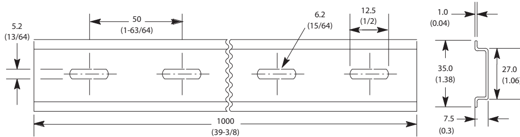
Figure 45 - Cat. No. 199-DR1 DIN Mounting Rail, Series B
