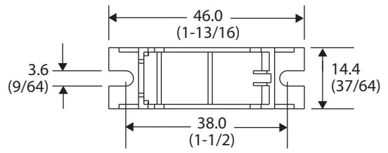
Figure 38 - Cat. No. 700-HN226
