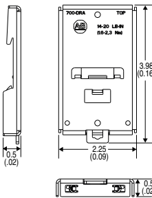
Figure 113 - Cat. No. 700-DRA DIN Rail Adapter
