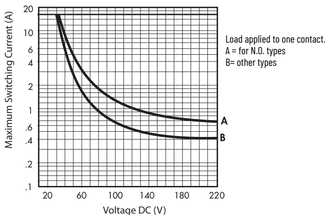
Figure 19 - Breaking capacity for DC-1 load at 600 cycles/hour
