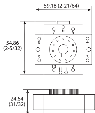
Figure 73 - Cat. No. 700-HN126
