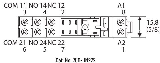
Figure 36 - Cat. No. 700-HN221, -HN222
