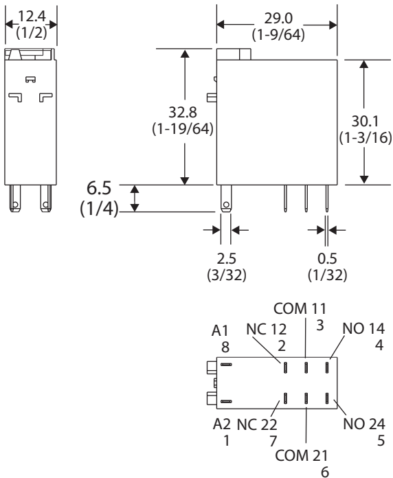
Figure 35 - Cat. No. 700-HK32_ (DPDT)
