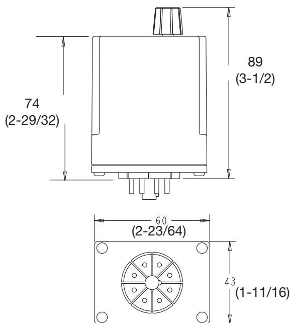
Figure 97 - 700-HT Relays
