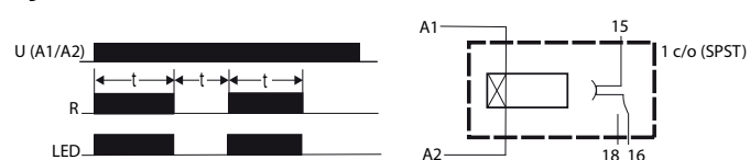
Figure 54 - Flasher
