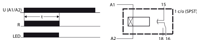
Figure 52 - One Shot
